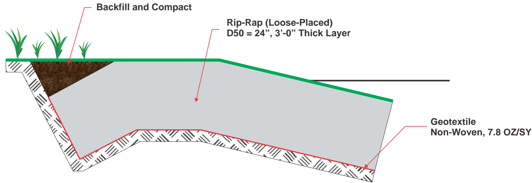
Rip-Rap Cross-Section Typical
