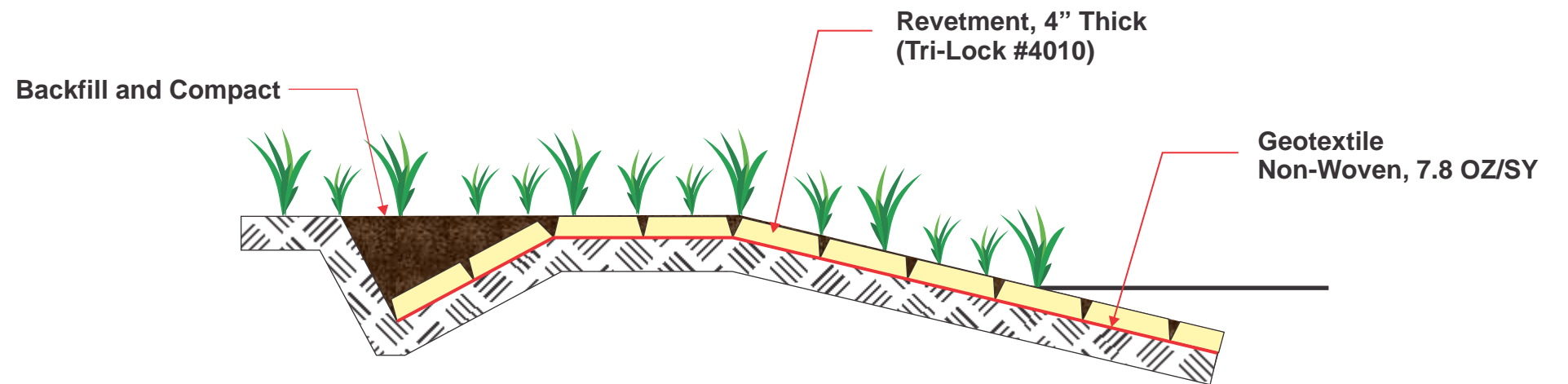
Tri-Lock Revetment Cross-Section, Typical
